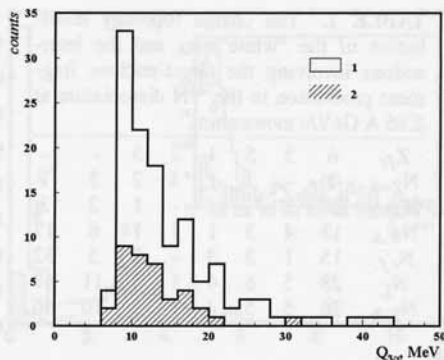
FIGURE 5. The invariant excitation energy Q_{3\alpha} distribution of three \alpha particles with respect to the ^{14}\text{N} ground state for the process ^{14}\text{N} \rightarrow 3\alpha + X . The following notation is used: 1) all the events of the ground state dissociation, 2) “white” stars.
