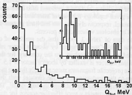
FIGURE 6. The invariant excitation energy Q_{2\alpha} distribution of \alpha particle pairs for the process ^{14}\text{N} \rightarrow 3\alpha + X . In the inset: a fraction of the distribution at 0-500 keV.
