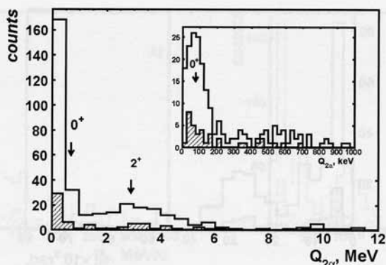
FIGURE 4. The invariant energy Q_{2\alpha} distribution of \alpha particle pairs in the {}^9\text{Be} \rightarrow 2\alpha fragmentation reaction at 1.2 A GeV energy. On the intersection: the Q_{2\alpha} range from 0 to 1 MeV. Arrows mark the {}^8\text{Be} nucleus levels ( 0^+ and 2^+ ). The outer contour corresponds to all events. The inner histogram is obtained for events, which accompanied by protons recoil of emulsion target (dashed area).
