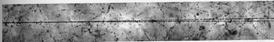
FIGURE 1. An event of the type of "white" star from the fragmentation of a relativistic {}^9\text{Be} nucleus into two He fragments in emulsion. The photograph was obtained on the PAVIKOM(FIAN) complex.
