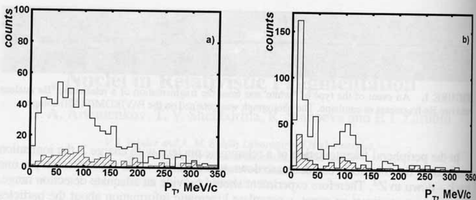
FIGURE 2. The P_T transverse momentum distribution of \alpha particles in the laboratory system (a), and the P_T^* momentum distribution in the c.m.s. of an \alpha particle pair (b). The outer contour corresponds to all events. The inner histogram is obtained for events, which accompanied by protons recoil of emulsion target (dashed area).
