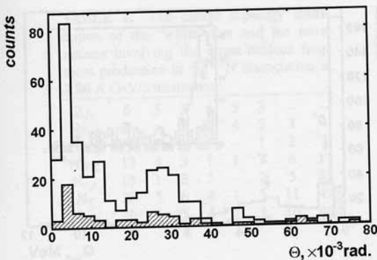
FIGURE 3. The opening \Theta angle distribution of \alpha particles in the {}^9\text{Be} \rightarrow 2\alpha fragmentation reaction at 1.2 A GeV energy. The outer contour corresponds to all events. The inner histogram is obtained for events, which accompanied by protons recoil of emulsion target (dashed area).
