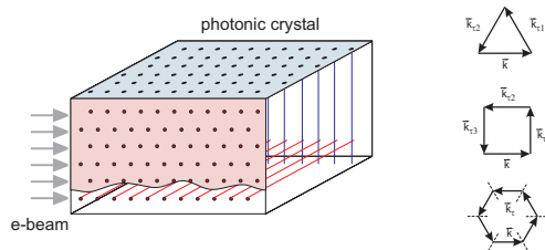
Figure 2: An example of photonic crystal with the thread arrangement providing multi-wave volume distributed feedback. Threads are arranged to couple several waves (three, four, six and so on), which appear due to diffraction in such a structure, in both the vertical and horizontal planes. The electronic beam takes the whole volume of photonic crystal.
